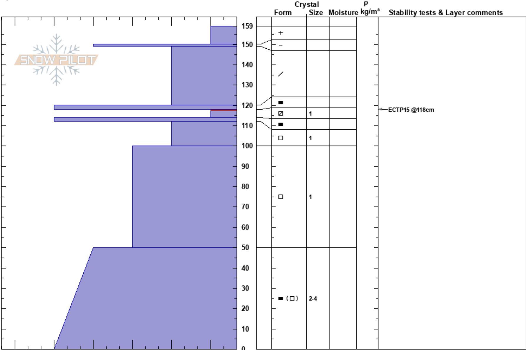
Notes: Crown Profile of a suspected snowmobile triggered avalanche 12/30/2020
